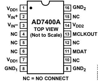
Figure 6. 16-Lead SOIC Pin Configuration
