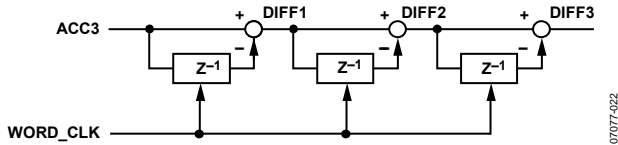
Figure 27. Differentiator
